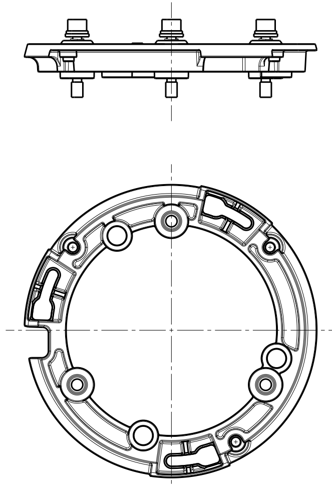
Attachment ring (For PTZ)
