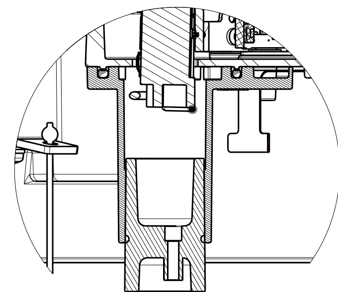
Detail C (1:1)
