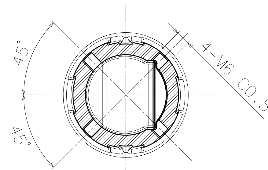
Sec A-A (1:1)
